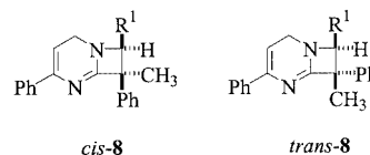
Figure 2. Azeto[1,2- a ]pyrimidines cis - 8 and trans - 8
