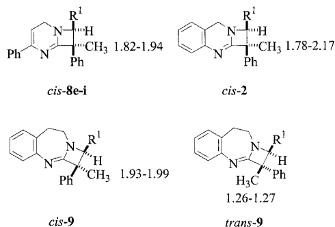
Figure 3. Selected 1 H NMR ( \delta , ppm) data for compounds cis - 8e–i , cis - 2 , cis - 9 and trans - 9
