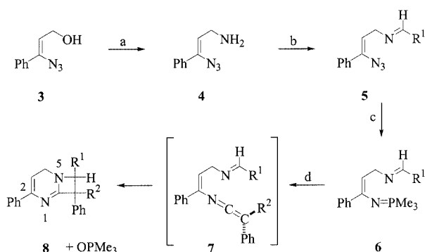
Scheme 1. Reagents and conditions: (a) (i) PPh 3 , EtO 2 CN=NCO 2 Et, phthalimide, THF, 0 °C 1 h, room temp. 36 h; (ii) N 2 H 4 ·H 2 O, THF/EtOH, room temp. 16 h, 50 °C 2 h; (b) R 1 CHO, MgSO 4 , room temp., 16 h; (c) PMe 3 , toluene, room temp., 30 min (d) R 2 PhC=C=O, toluene, room temp., 30 min
