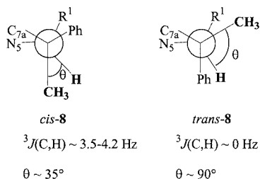
Figure 4. Newman projection of cis - 8 ( \text{R}^2 = \text{CH}_3 ) and trans - 8 ( \text{R}^2 = \text{CH}_3 ) along the C-6–C-7 bond
