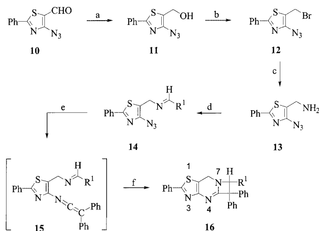
Scheme 2. Reagents and conditions: (a) NaBH 4 , THF/Et 2 O, 0 °C → room temp., 12 h; (b) PPh 3 Br 2 , Et 3 N, benzene, room temp., 12 h; (c) (i) potassium phthalimide, DMF, 80 °C, 12 h; (ii) N 2 H 4 ·H 2 O, THF/EtOH, room temp. 16 h, 60 °C 1.5 h; (d) R 1 CHO, MgSO 4 , Et 2 O, room temp., 16 h; (e) (i) PMe 3 , toluene, room temp., 30 min; (ii) Ph 2 C=C=O, toluene, room temp., 15 min; (f) toluene, reflux, 1 h
