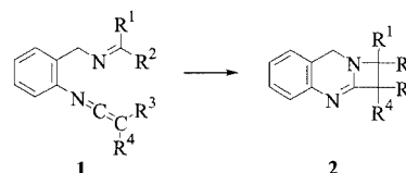
Figure 1. Intramolecular [2+2] cycloaddition of imino-ketenimines on an ortho -benzylic scaffold
