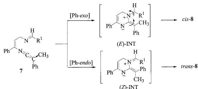
Figure 5. Mechanism for the conversion 7 → 8
